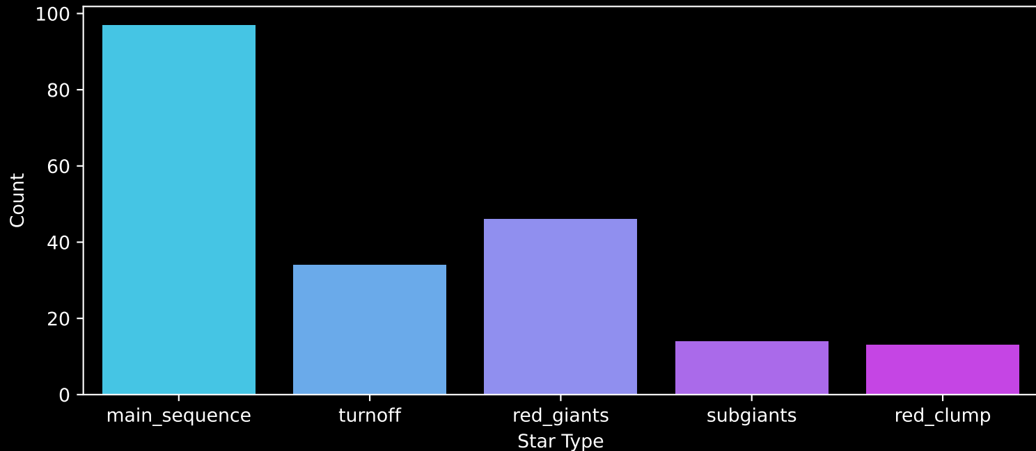
APOGEE DR17 Field: [203+30_MGA] Count plot of Star Type
