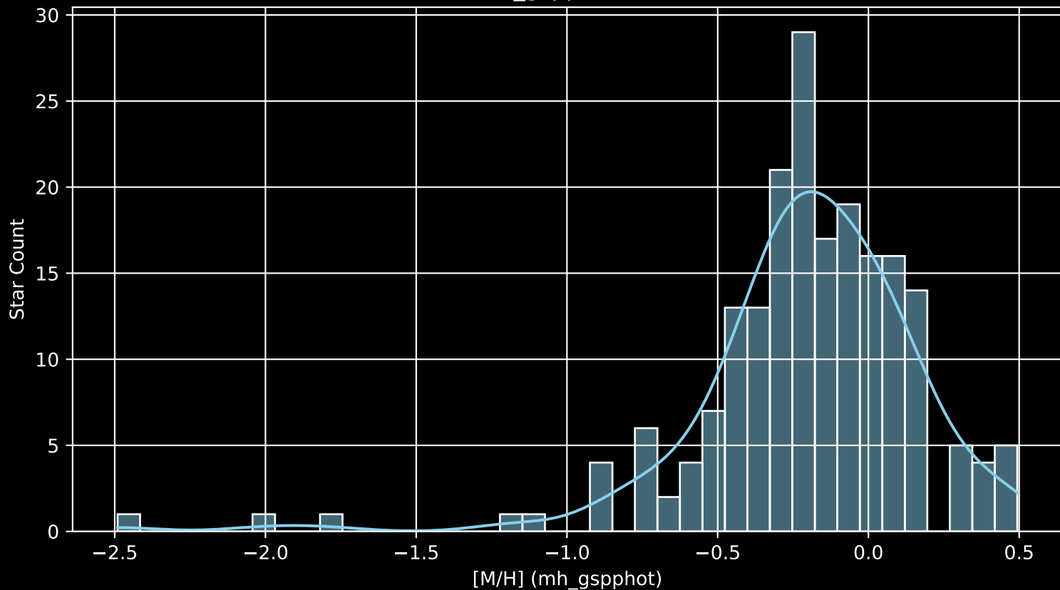
APOGEE DR17 Field: [203+30_MGA [M/H] (mh_gspphot) (n= 200)
