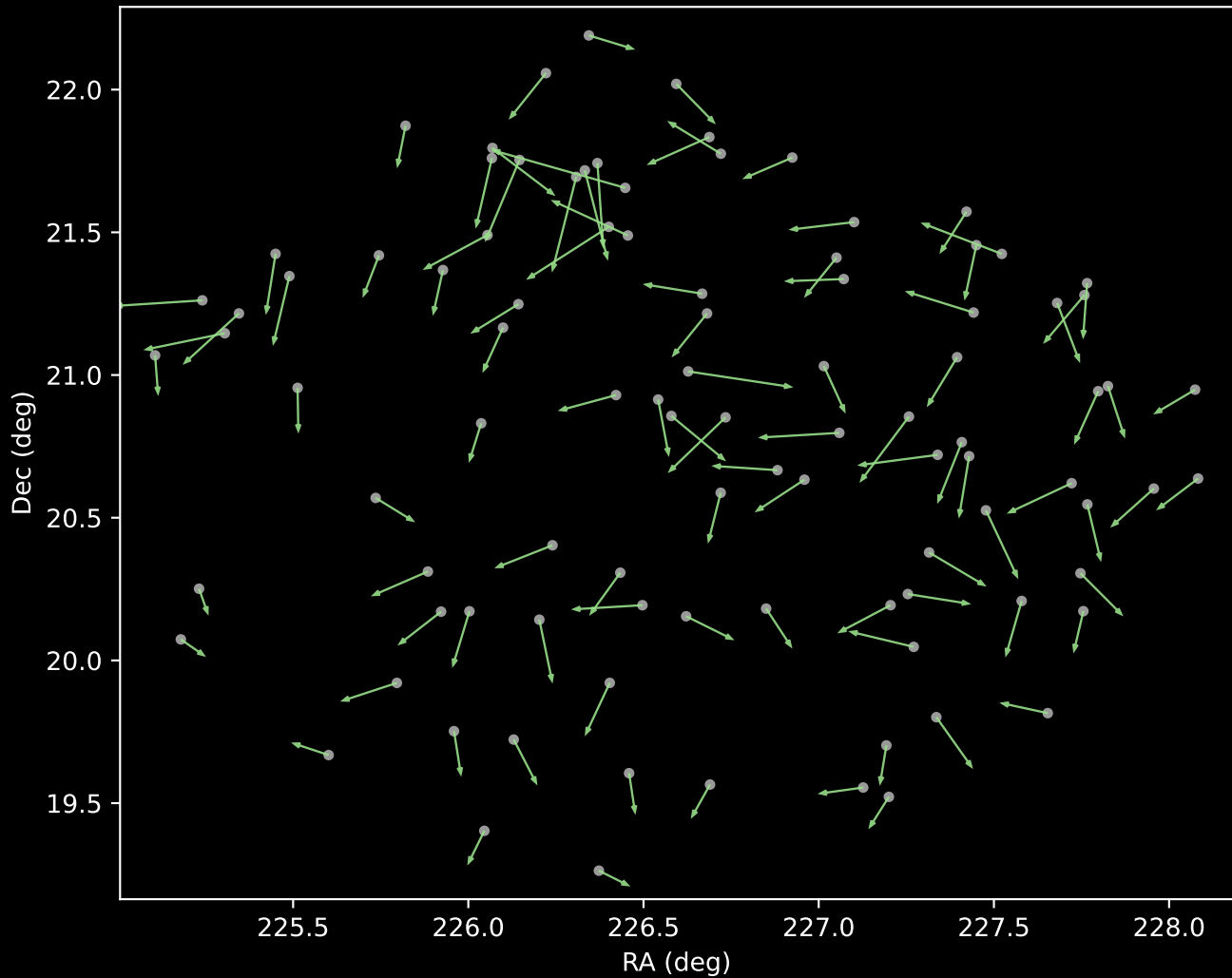
APOGEE DR17 Cluster 5 Proper Motion Vectors (n=97)
