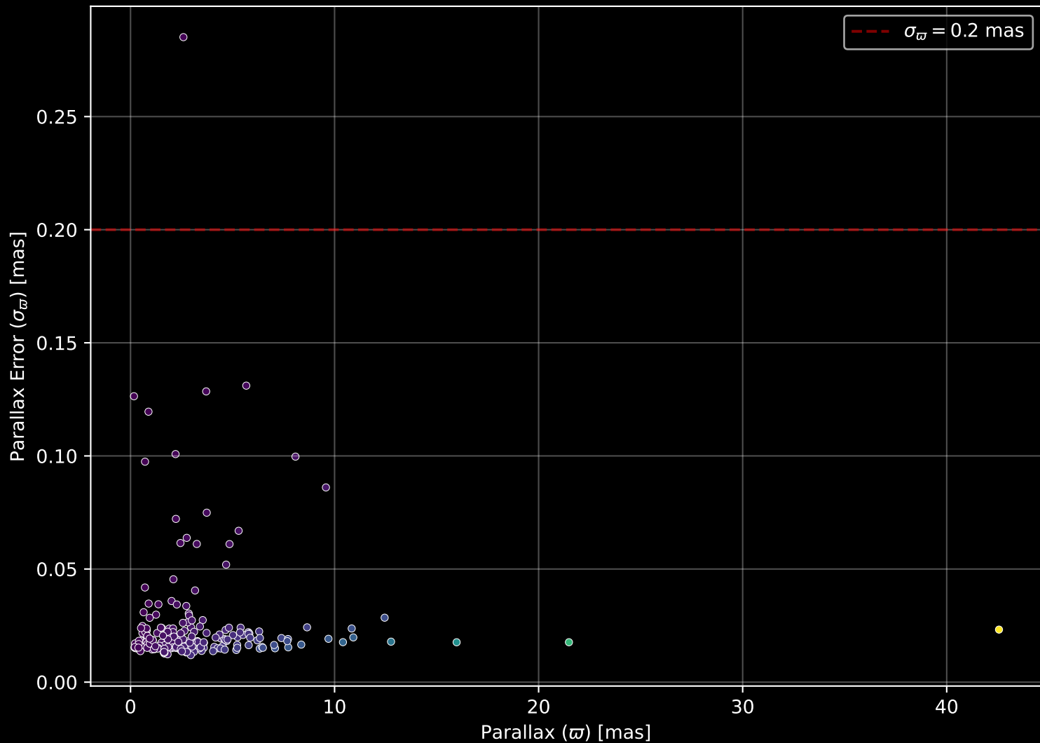
APOGEE DR17 Field: [203+30_MGA] Parallax Quality (n= 204)
