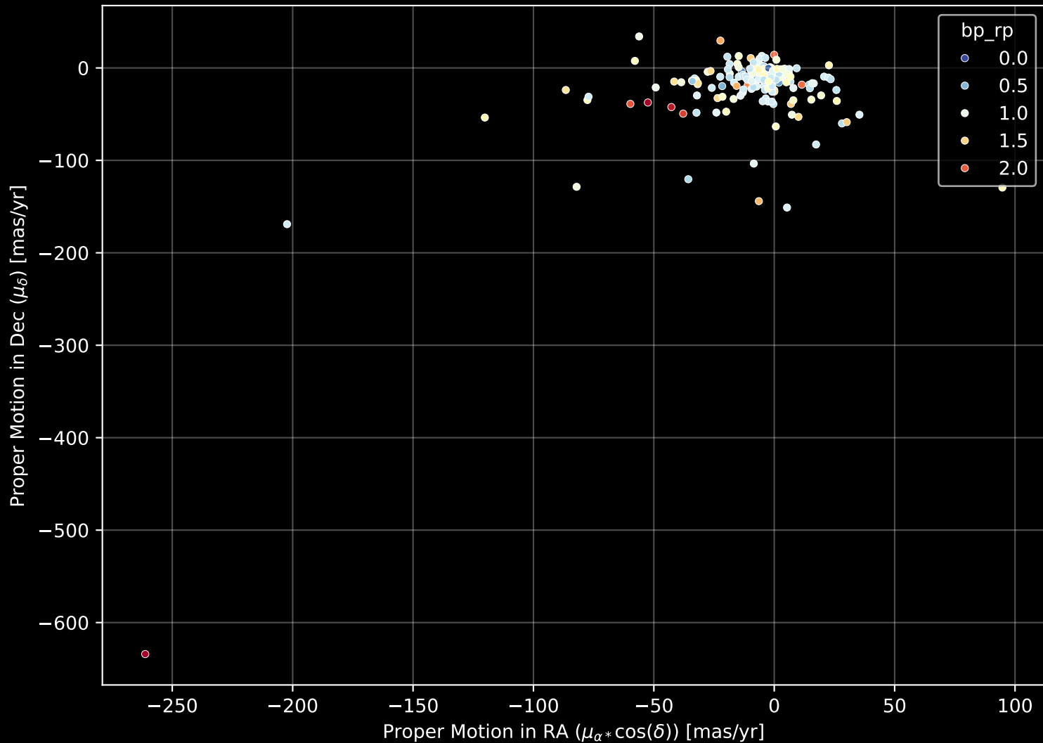
APOGEE DR17 Field: [203+30_MGA] Proper Motion Diagram (n= 204)
