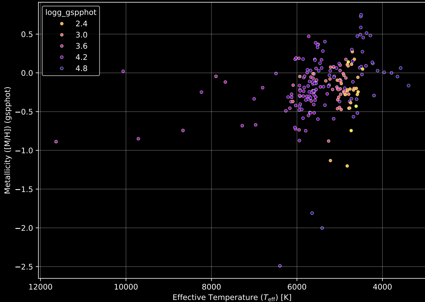
APOGEE DR17 Field: [203+30_MGA] Stellar Population Parameters (n= 204)
