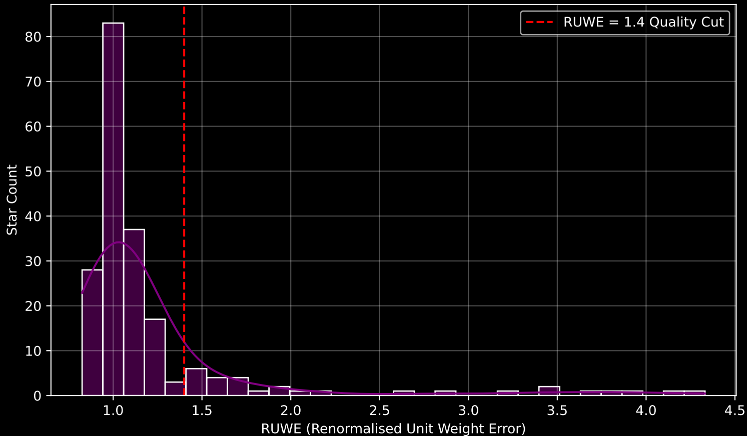
GAPOGEE DR17 Field [203+30_MGA] RUWE Distribution (n= 197)
