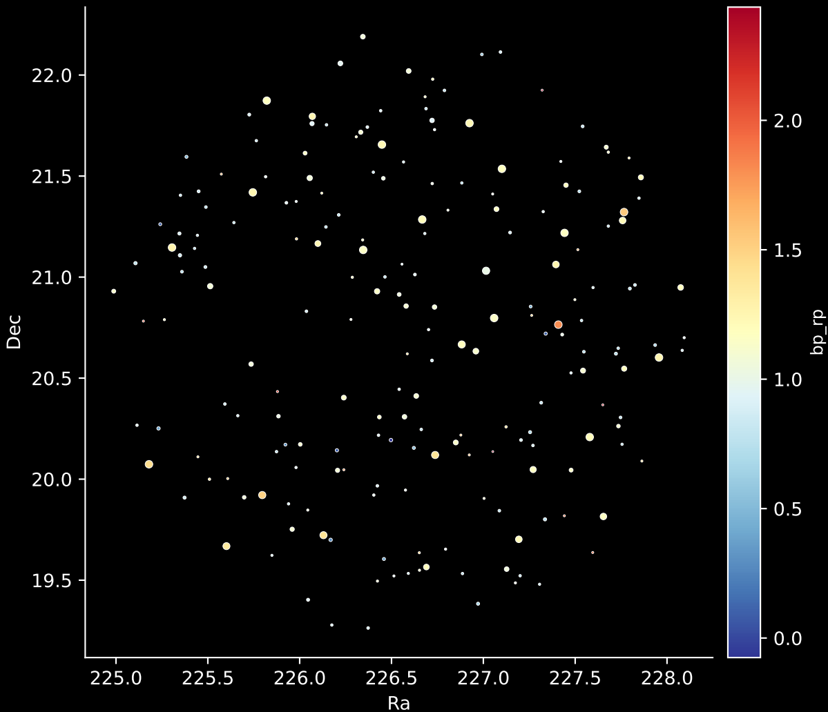
APOGEE DR17 Field: [203+30_MGA] Stars: 204
